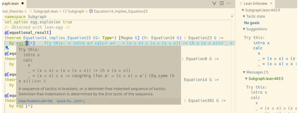
FIGURE 12. Example of the egg tactic reconstructing a proof in human-readable form with the help of calcify (invoked by the special syntax egg? ).
