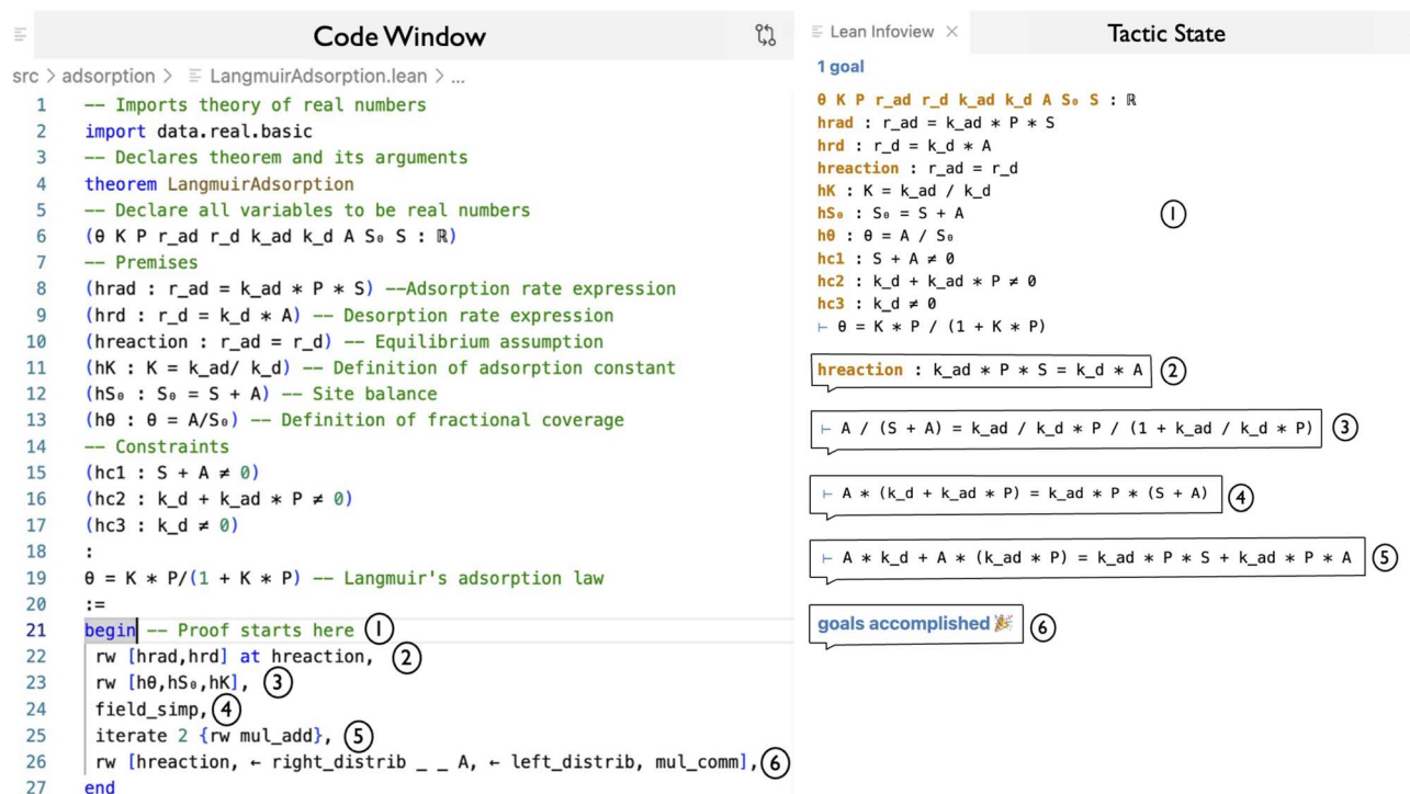
Fig. 1 A formalization of Langmuir's adsorption model, shown as screenshots from Lean operating in VS Code. The left side of the figure shows the "Code Window," while the right side shows variables and goals at each step in the "Tactic State". When the user places the cursor at one of the numbered locations in the "Code Window," VS Code displays the "Tactic State" of the proof. Lean allows the use of Unicode symbols, so we use " S_0 " to represent the total concentration of adsorption sites without needing underscores. The turnstile symbol represents the state of the goal after each step. As each tactic is applied, hypotheses and/or goals are updated in the tactic state as the proof proceeds. For clarity, we only show the hypothesis that changes after a tactic is applied and how that changes the goal. As an example, the goal state is the same in steps 1 and 2 since the first tactic rewrites (rw) the equation of adsorption ( h_{\text{rad}} ) and desorption ( h_{\text{rd}} ) into the premise that equilibrium ( h_{\text{reaction}} ) exists. Next, we rewrite (rw), simplify (field_simp), and otherwise rearrange the variables to exactly equal the goal state (steps 3–5). When the proof is finished, a celebratory message and party emoji appears (6).
